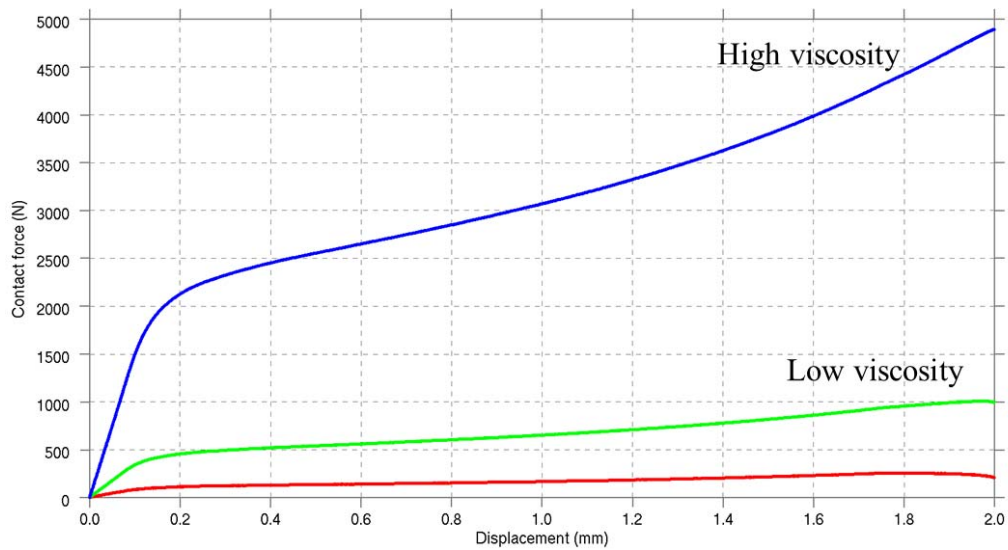
Fig.7: Contact force generated in models with different axial resistive forces
