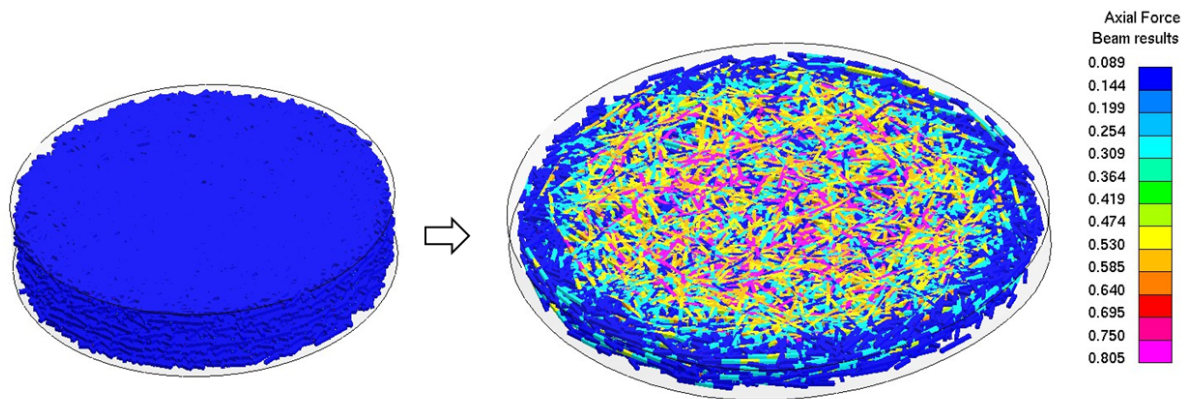
Fig.6: Deformation behaviour and axial forces in beam elements
