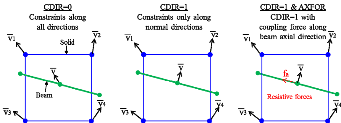
Fig.1: 3 types of coupling option in CBIS
