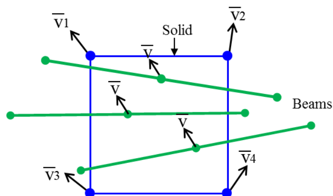
Fig.3: Constraint of multiple beam elements in one solid element
