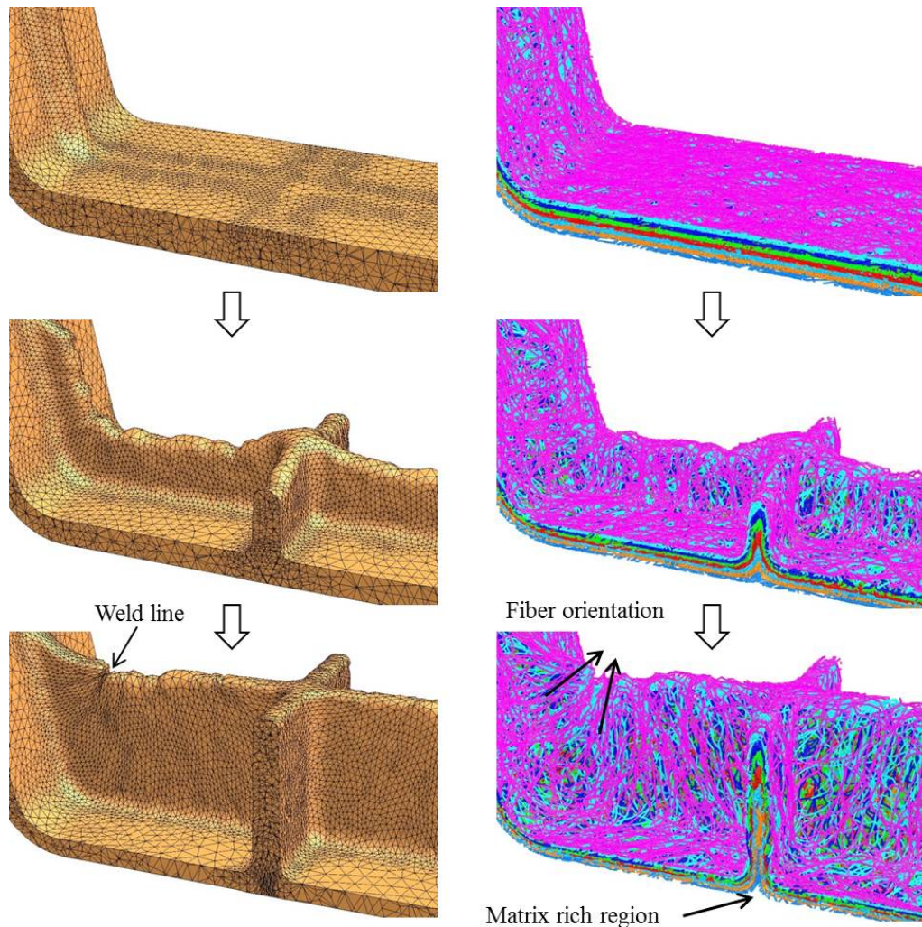
Fig.11: EFG r-adaptive mesh refinement and beam orientation behaviour
