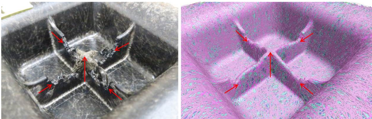
Fig.14: Formation of ribs and weld lines near the final punch stroke
