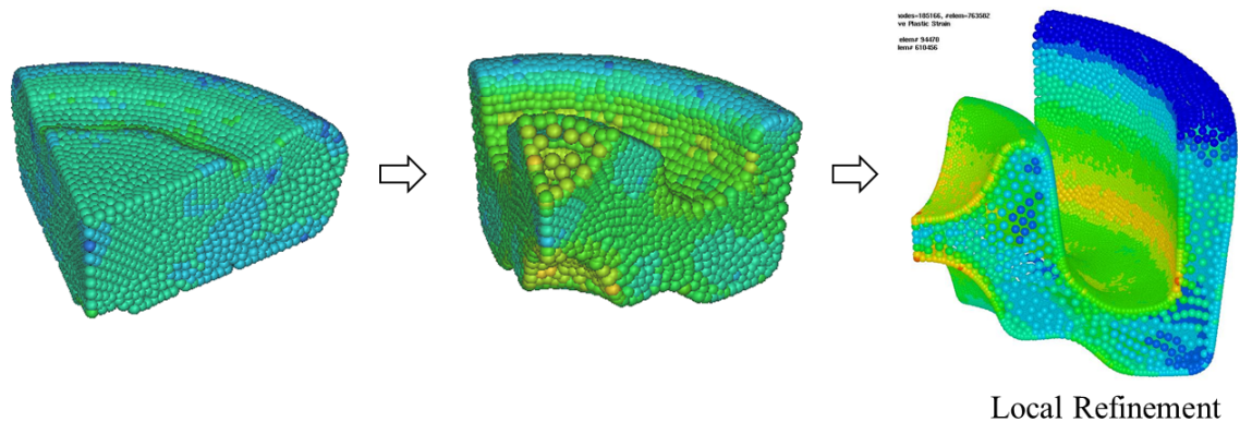
Fig.2: 3D forging simulation example using 3D adaptive EFG
