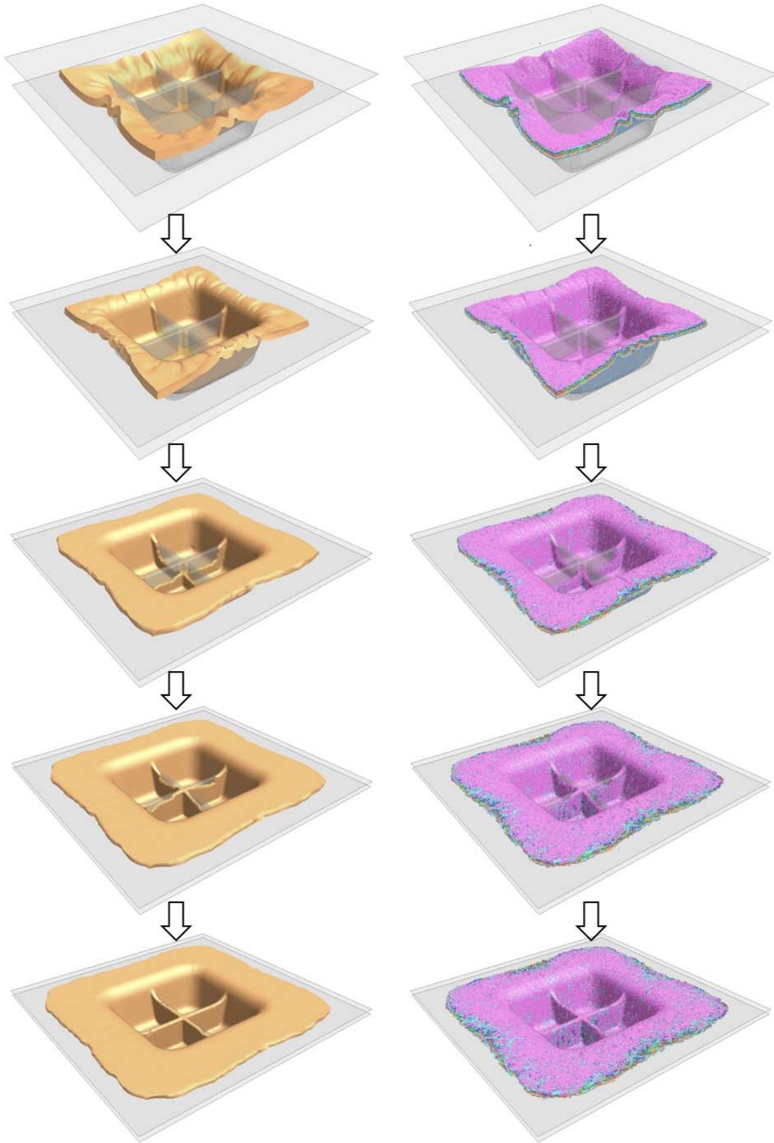
Fig.10: Deformation behaviour of solids as matrix (left) and beams as fibers (right)
