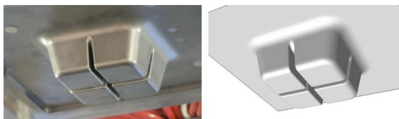
Fig.12: Punch shape used in experiment and LS-DYNA
