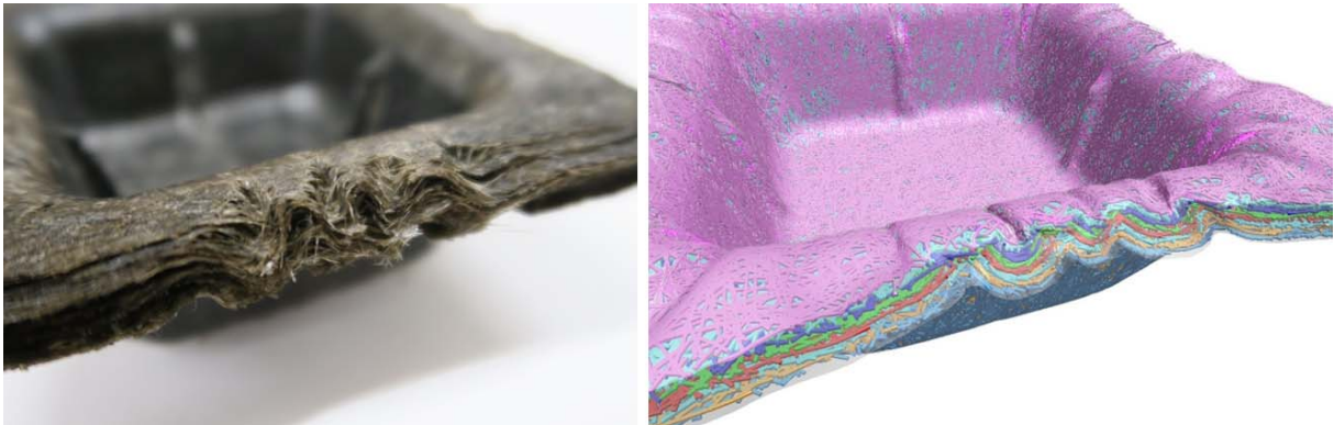
Fig.13: Charge wrinkling mid-way through the punching process
