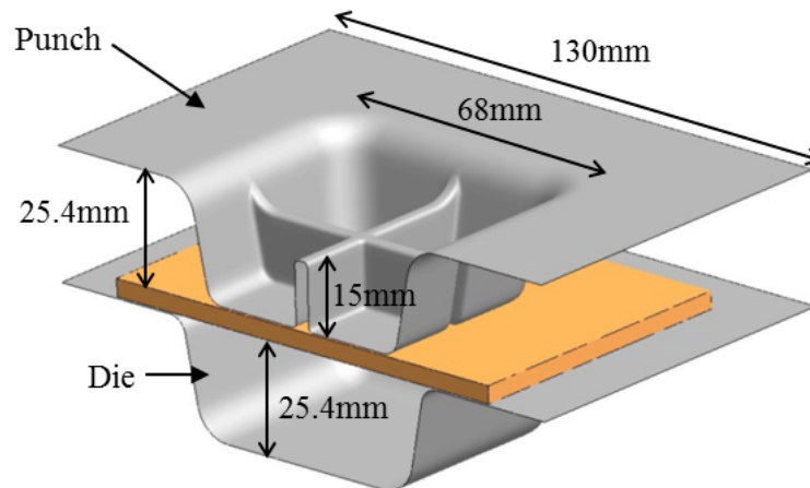
Fig.9: Compression molding model to form cross-rib shaped component
