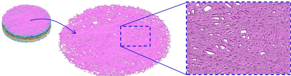
Fig.5: Eight layer model made of beam elements with 2D random orientation
